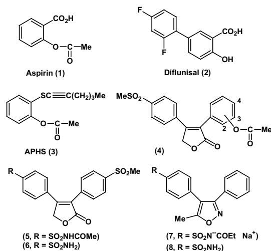
Figure 1. Some representative cyclooxygenase (COX) inhibitors.
