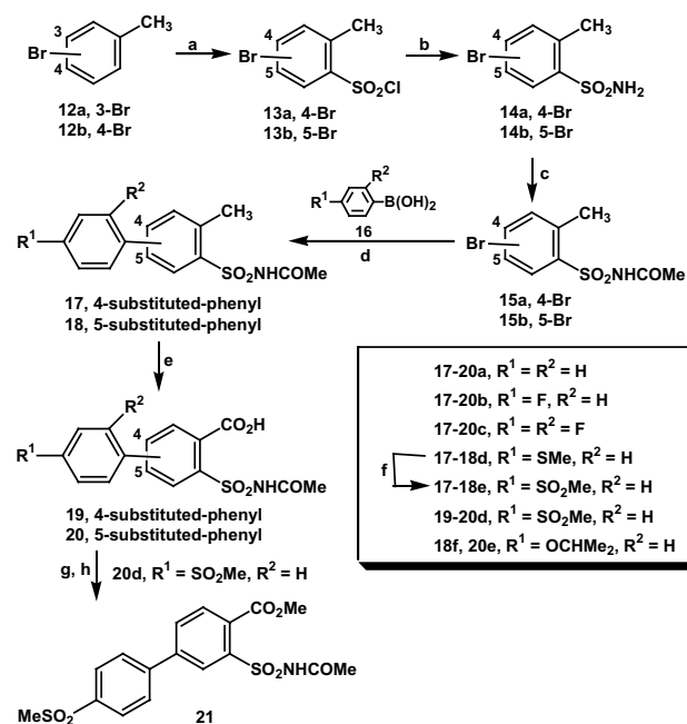
Scheme 2. Reagents and conditions: (a) ClSO 3 H, CHCl 3 , 0 °C, 4 h; (b) 30% w/v NH 4 OH, dioxane, 0 °C, 6 h; (c) Ac 2 O, DMAP, pyridine, 25 °C, overnight; (d) Pd(PPh 3 ) 4 , Na 2 CO 3 , THF, reflux, 5 h; (e) KMnO 4 , 0.5 N NaOH, 60 °C, 4 h; (f) Oxone®, THF, MeOH, H 2 O, 25 °C, 2 h; (g) MeOH, H 2 SO 4 , 80 °C, overnight; (h) Ac 2 O, pyridine, DMAP, 25 °C, overnight.
