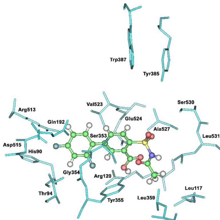
Figure 2. Docking of N -acetyl-2-carboxy-4-(2,4-difluorophenyl)benzenesulfonamide ( 19c ) (ball-and-stick) in the active site of murine COX-2. Hydrogens atoms of the amino acid residues have been removed to improve clarity.
